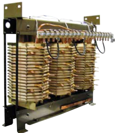
Federal Pacific three-phase, 80 kVA 480 delta input and total of 18 individual single-phase 440V outputs.
