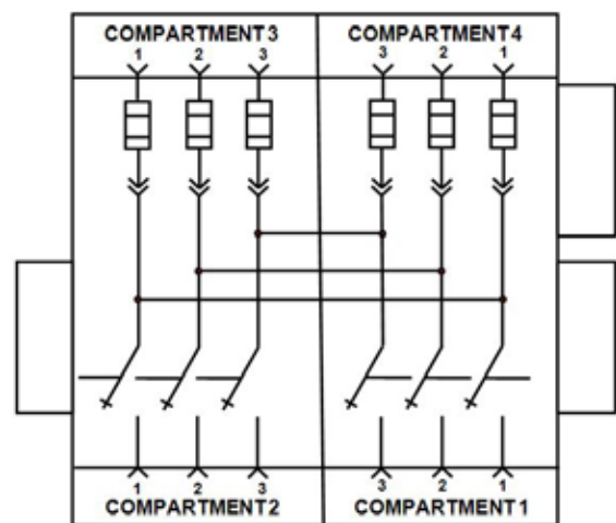
Figure 3 – Circuit Diagram for typical ATPSE-9 Dead-Front Pad-Mounted Switchgear, with three-phase Auto-jet® switches in compartments 1 and 2, and a three-phase set of fuses in compartments 3 and 4.
