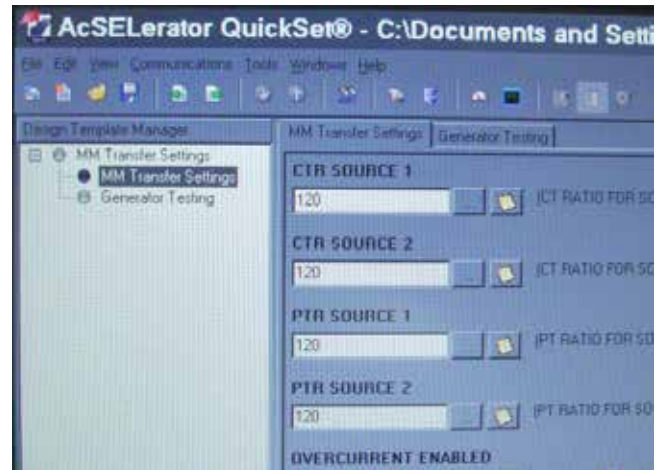
Figure 11. The Field Selectable functions are found in the “MM Transfer Settings” screen within the imbedded software furnished with the pad-mounted switchgear. Two drop-down menus are provided. When the service is from two utility sources the functions are included on the “MM Transfer Settings”. When the alternate source is a standby generator, additional field-selectable functions are provided and these are found in the “Generator Testing” tab.
