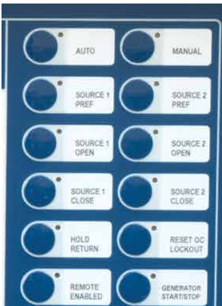
Figure 8. Twelve (12) interactive soft keys provide Local Operation capability on the faceplate of the SEL-451 relay. With Local Operation capabilities, operating personnel can perform switching operations and other key functions with direct interface on the relay.
