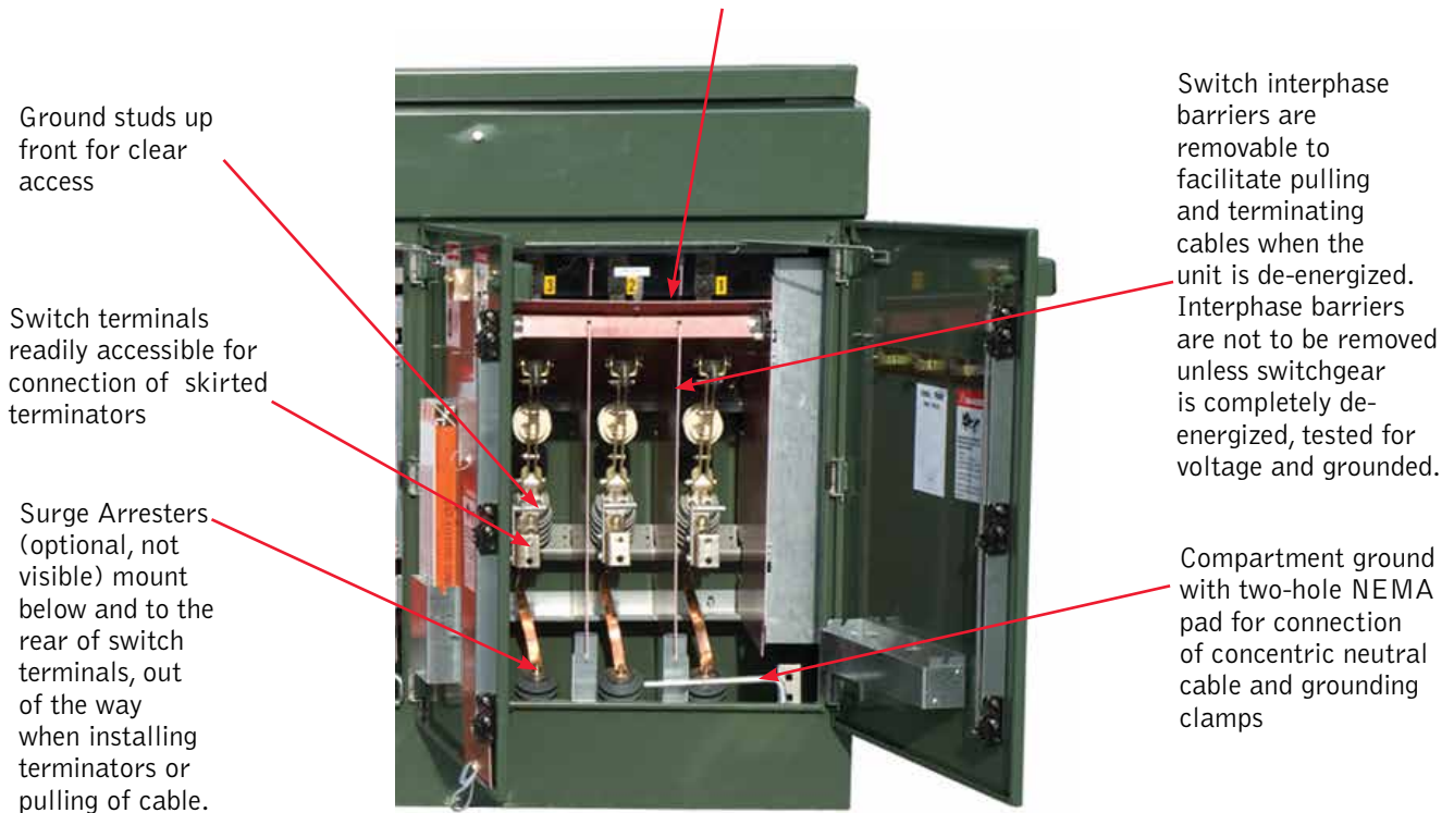
Live-front switches utilize conventional, skirted terminators and eliminate the need for costly, difficult to handle 600-ampere elbow connectors.
