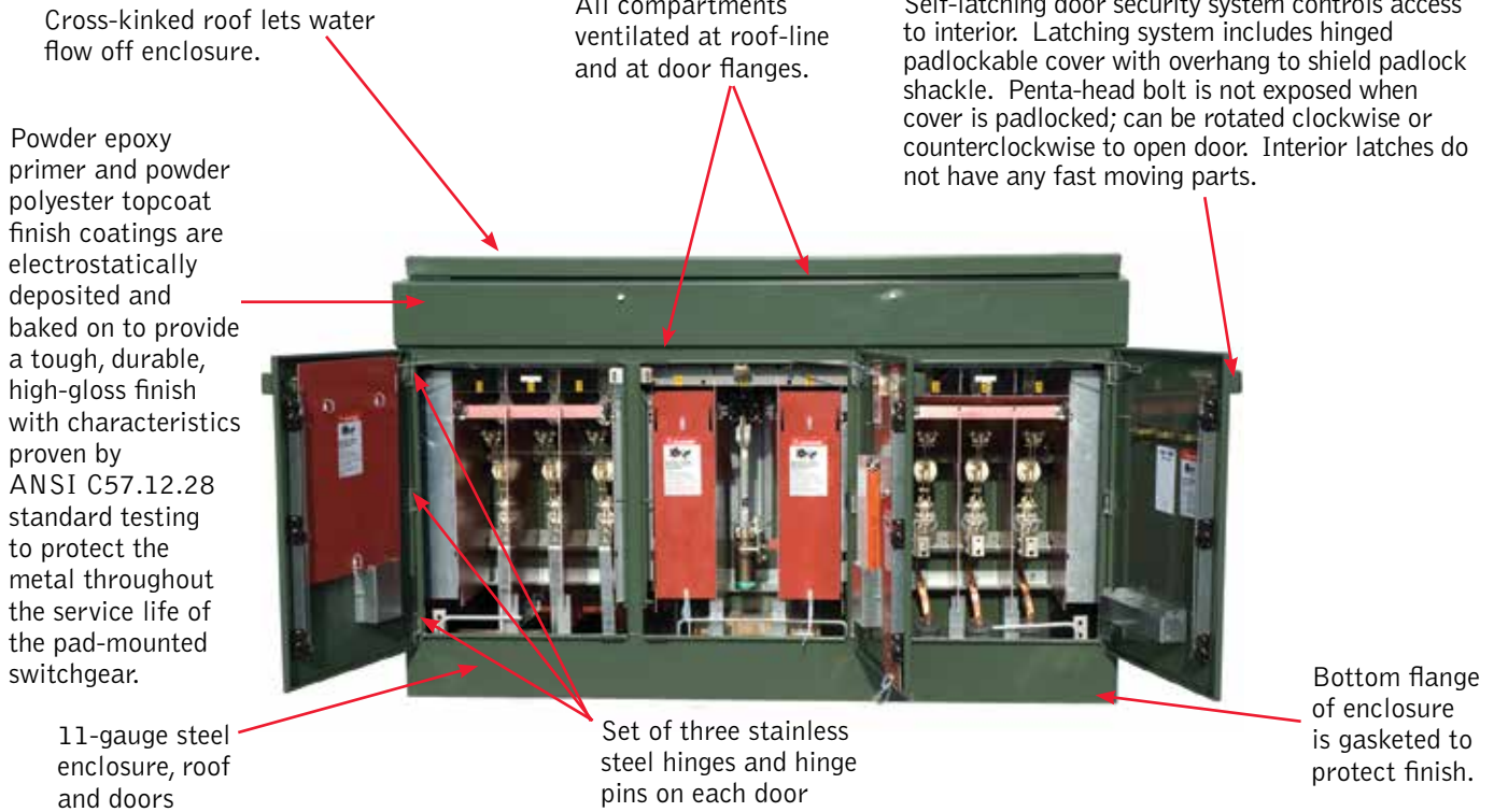
Enclosure integrity and security is assured with Federal Pacific Type PSI/II Pad-mounted Switchgear.
