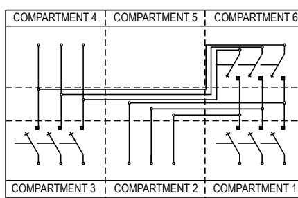
Drawing Number 37-0146-023 — Bus-Tie Configuration with two outgoing bus-only tap circuits
