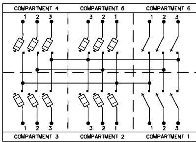
Drawing Number 37-0146-001 — Two incoming switches and four fused feeders
