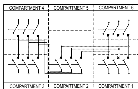
Drawing Number 37-0146-033 — Bus-Tie Configuration with two switched feeders
