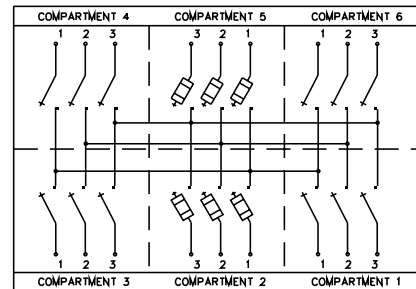
Drawing Number 37-0146-003 — Four incoming switches and two fused feeders
